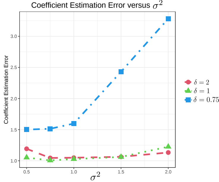
Figure 3: Coefficient estimation errors for Algorithm 1 with different input \sigma^2 based on 100 replicates.
