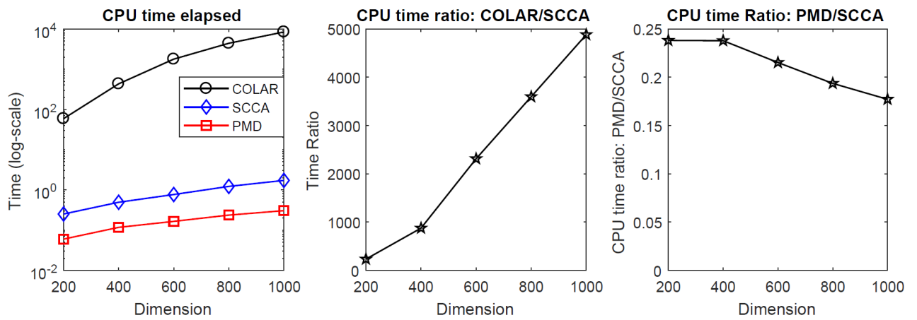
Figure 1. Elapsed CPU time for fitting each method. Left panel summarizes the averaged time (in log-scale) for each method to fit one data set with tuning based on five candidate tuning parameters. The averaged CPU time elapsed for each methods are (in seconds): 59.06 (COLAR), 0.25 (SCCA) and 0.06 (PMD) when p = q = 200 ; and 8419.3 (COLAR), 1.72 (SCCA) and 0.31 (PMD) when p = q = 1000 . The middle and right panels summarize the computing time ratios of COLAR versus SCCA and PMD versus SCCA.
