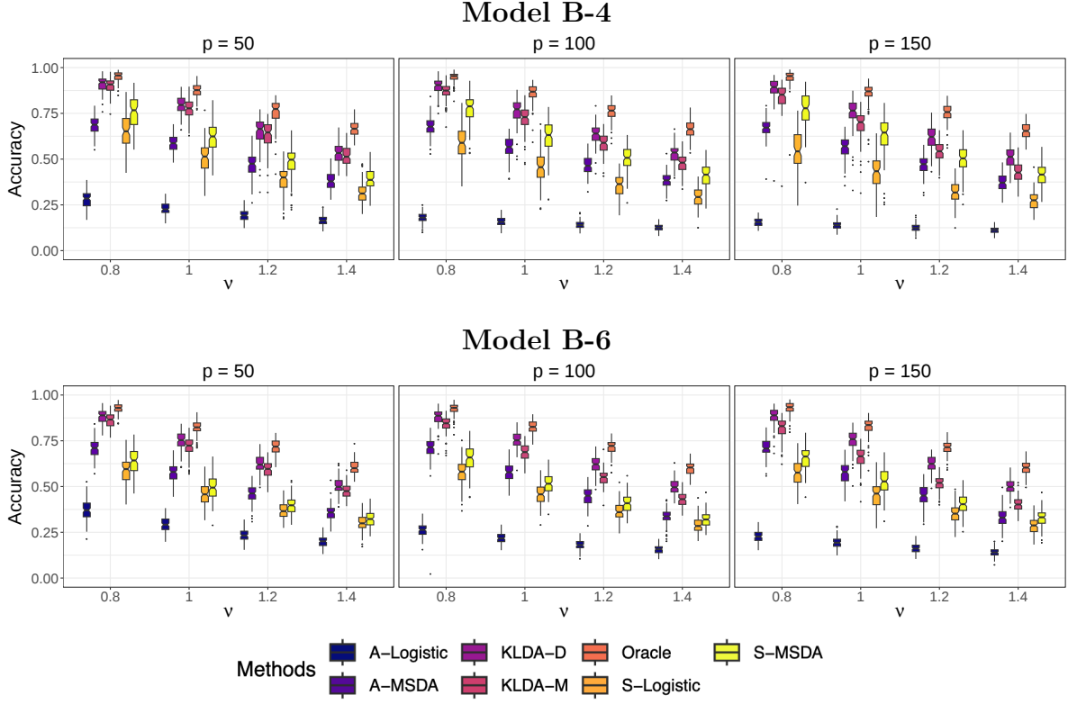
Figure 2: Prediction accuracy over 100 independent replications under Model B-4 and Model B-6 with (p, \nu) \in \{50, 100, 150\} \times \{0.8, 1.0, 1.2, 1.4\} .
